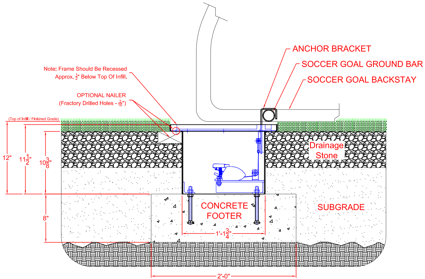
SE790 - SOCCER GOAL ANCHOR FRAME INSTALLATION DETAIL (Elevation View)
