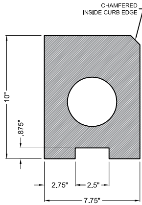
PART # SEFLEXLJ1
