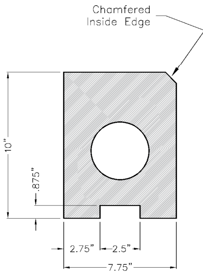
FlexEdge™ Rubber Long Jump Pit Curb System - No Ledge, 26'
