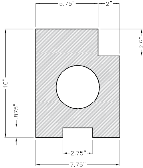
FlexEdge™ Rubber Long Jump Pit Curb System w/ Cover Ledge, 23' (Aluminum Pit Cover Set Sold Separately)
