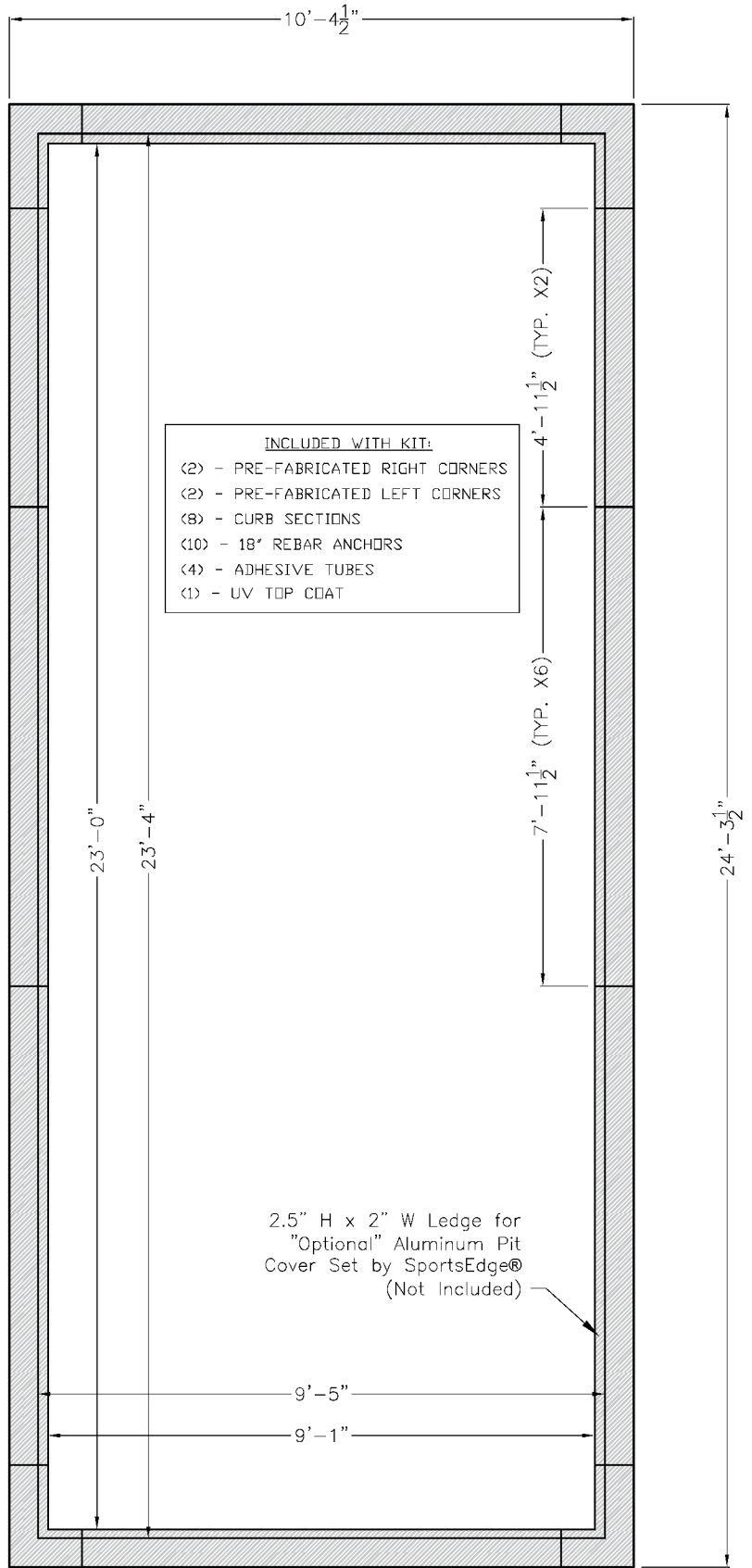
FlexEdge™ Rubber Long Jump Pit Curb System w/ Cover Ledge, 23' (Aluminum Pit Cover Set Sold Separately)
