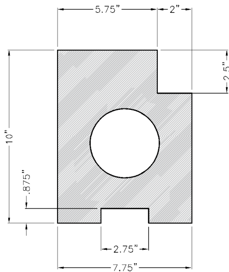
FlexEdge™ Rubber Long Jump Pit Curb System w/ Cover Ledge, 26' (Aluminum Pit Cover Set Sold Separately)
