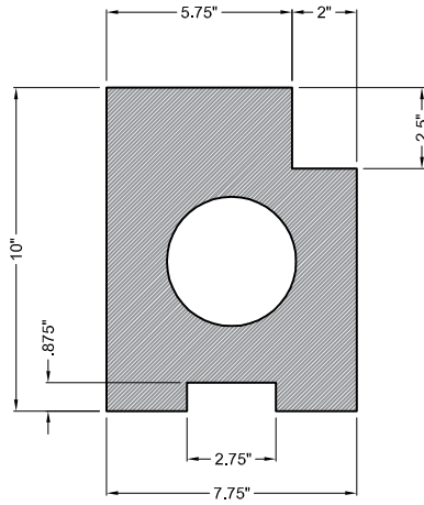
PART # SEFLEXLJ2
