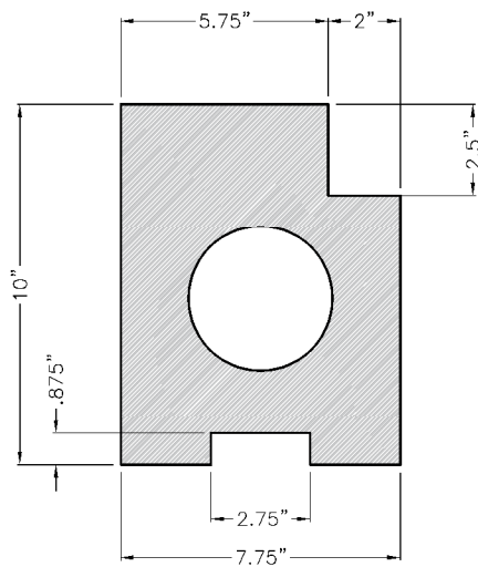
FlexEdge™ Rubber Long Jump Pit Curb System w/ Cover Ledge, 29' (Aluminum Pit Cover Set Sold Separately)
