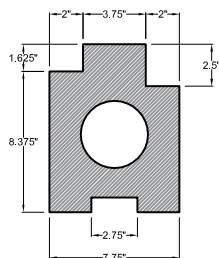
PART # SEFLEXLJ3B (SECTION "B" - QTY. X6)
