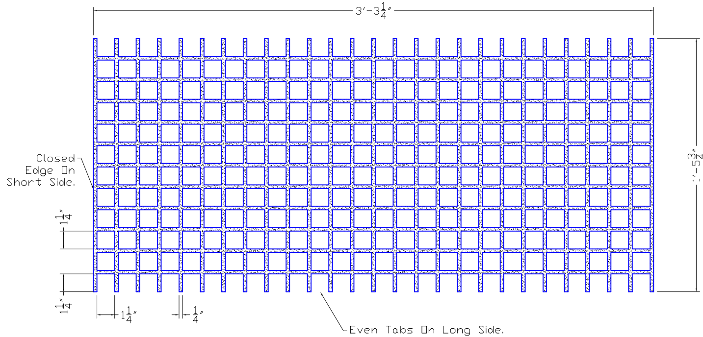
SportsEdge® FlexEdge® Sand Catcher Fiberglass Grate (Top View)
