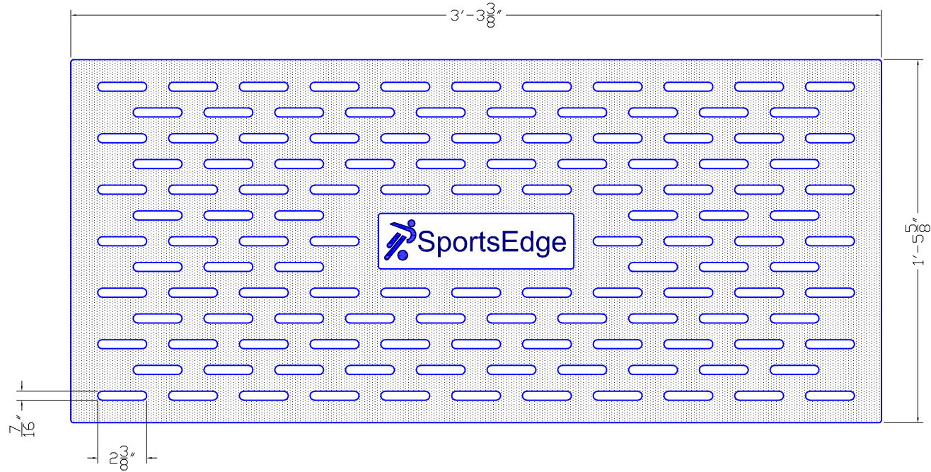
SportsEdge® FlexEdge® Sand Catcher Rubber Mat (Top View)
