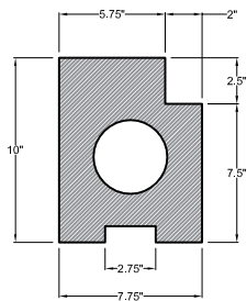
PART # SEFLEXLJ2 (SECTION "C" - QTY. X2)
