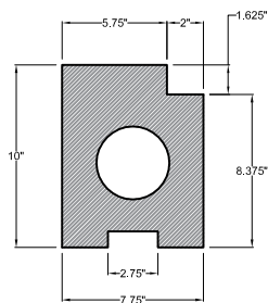
PART # SEFLEXLJ3A (SECTION "A" - QTY. X6)
