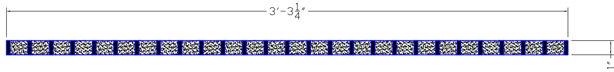
SportsEdge® FlexEdge® Sand Catcher Fiberglass Grate (Side View)
