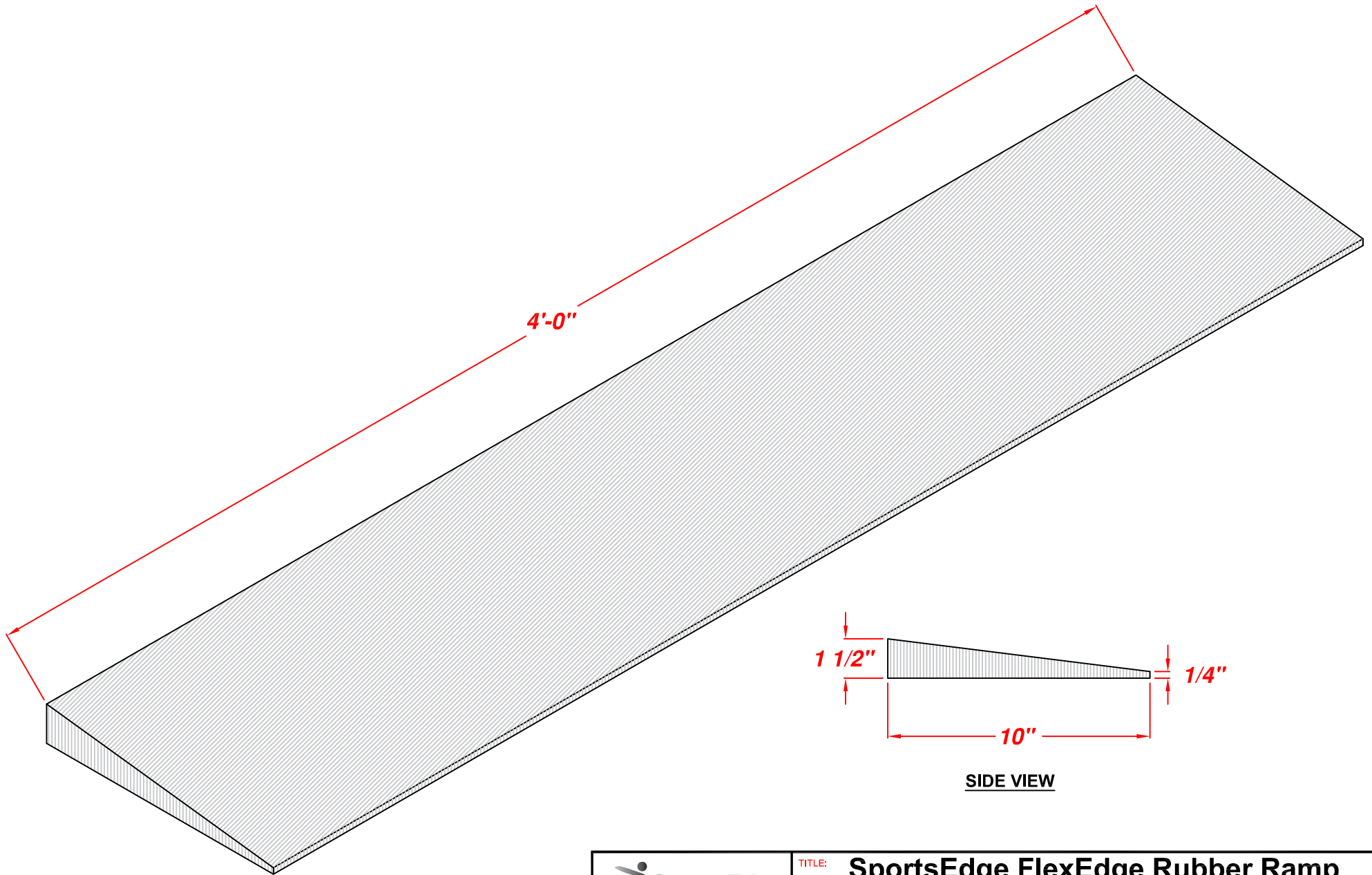
ISOMETRIC VIEW
