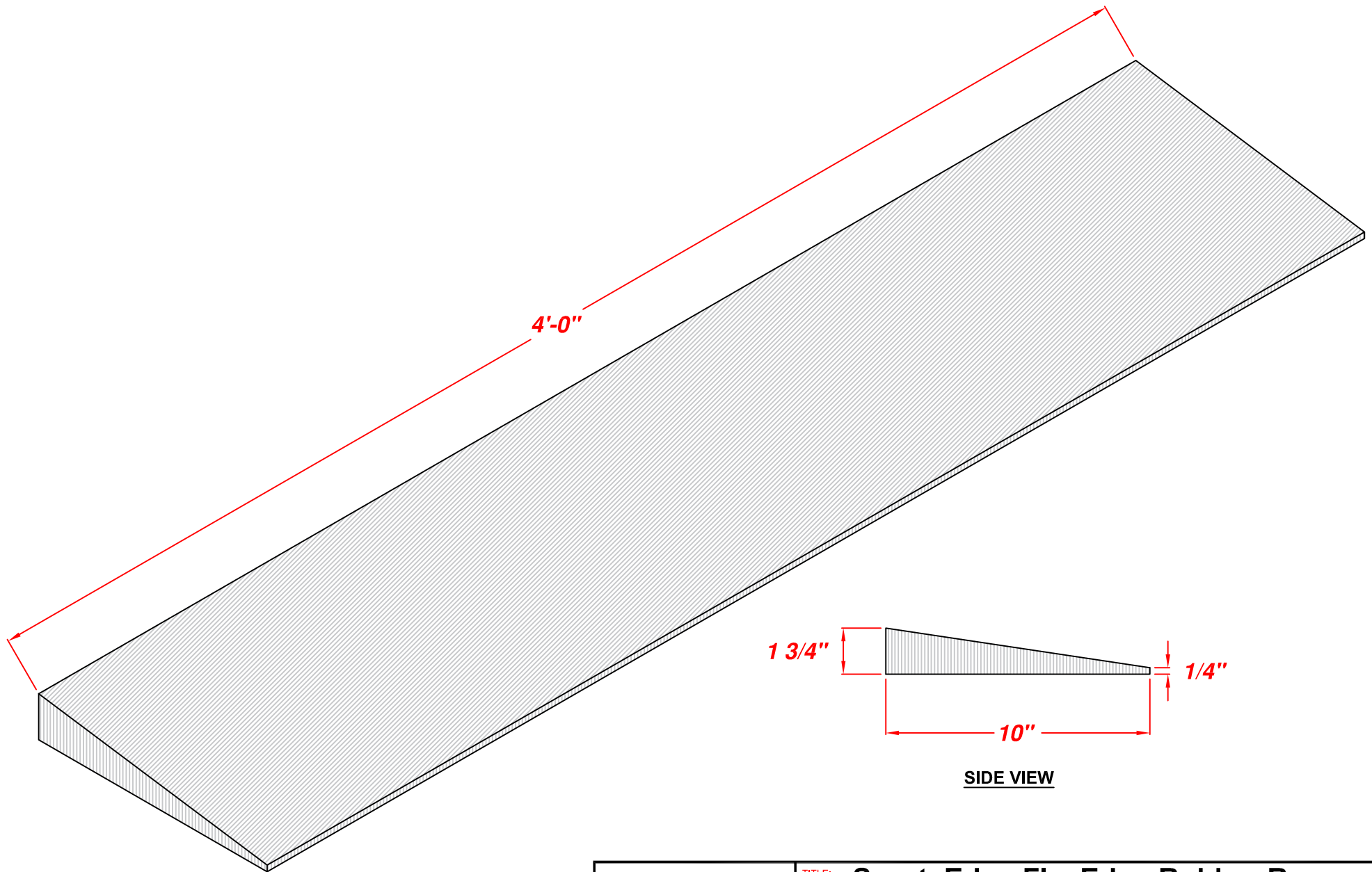
ISOMETRIC VIEW
