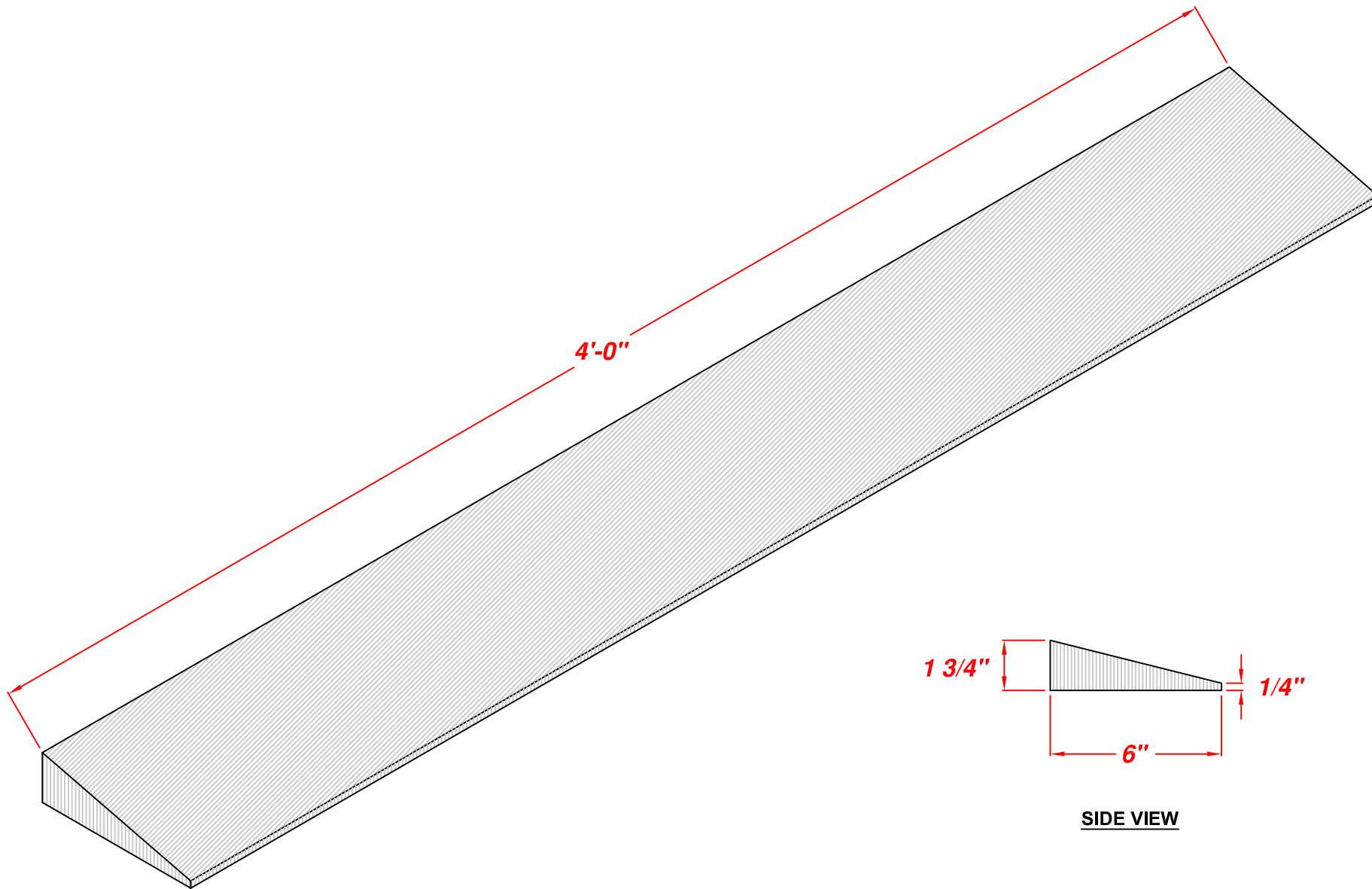
ISOMETRIC VIEW
