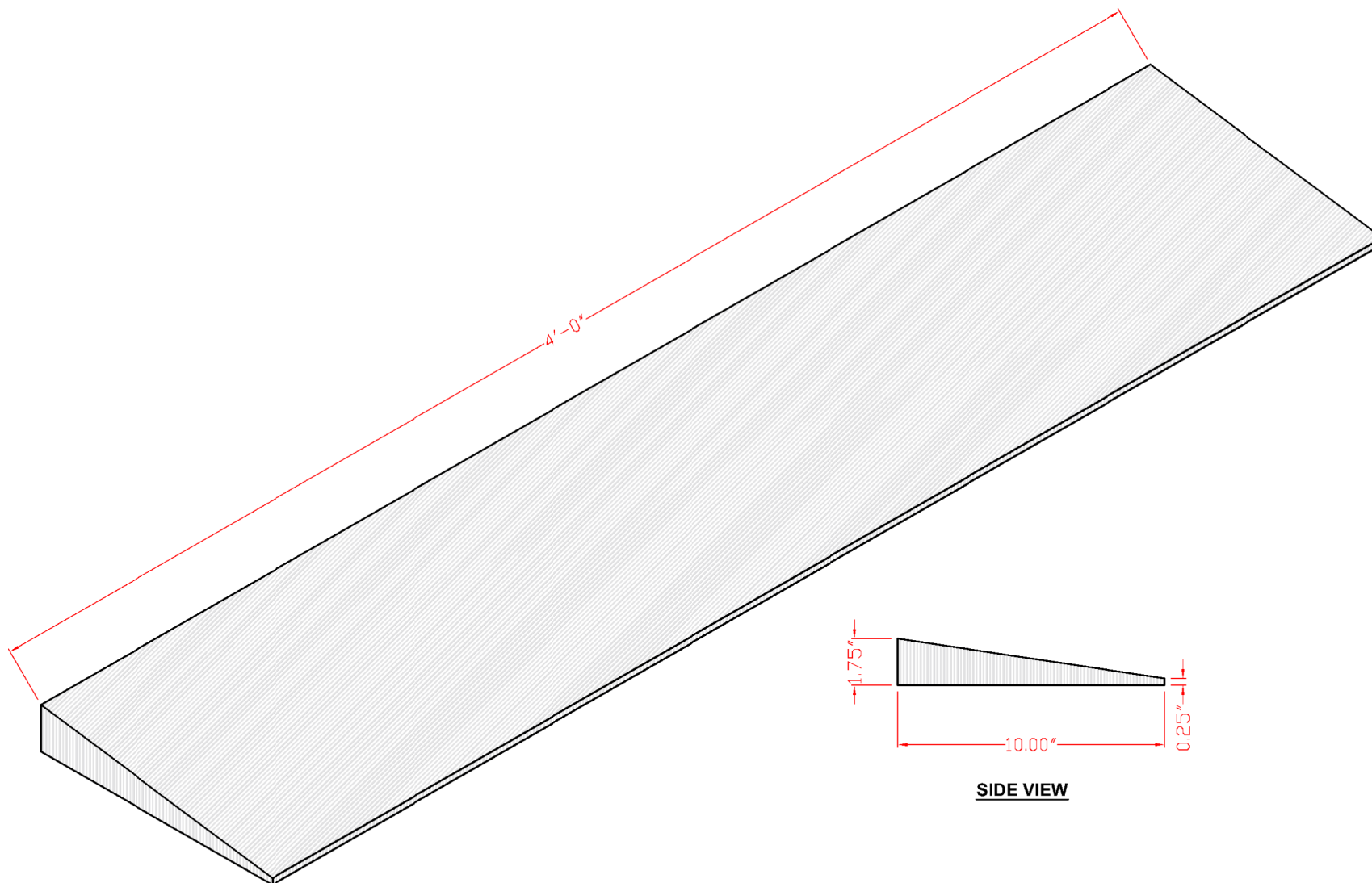
ISOMETRIC VIEW
