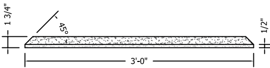
END VIEW
