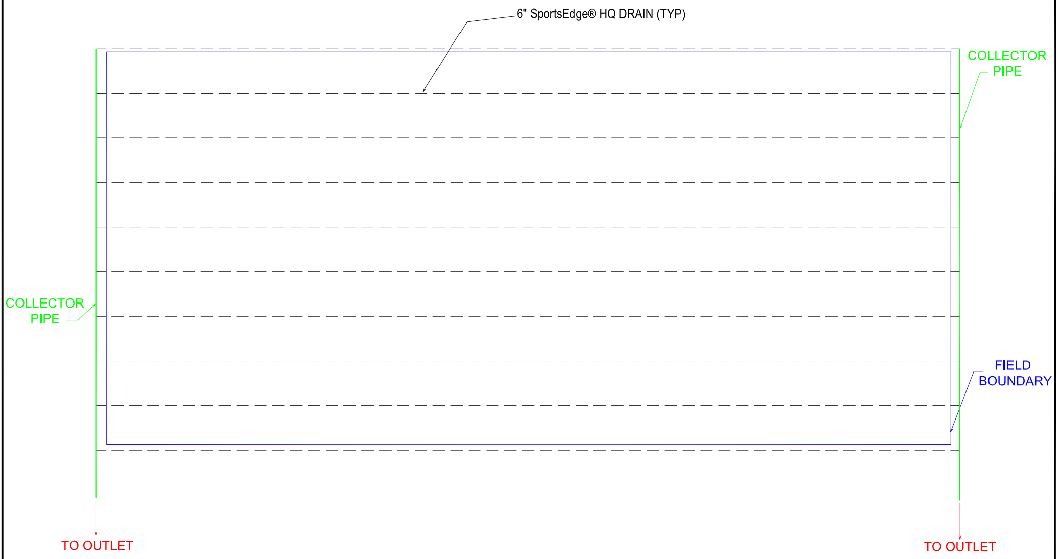
EXAMPLE LAYOUT SEHQ6 VERTICAL INSTALL- LONGITUDINAL
