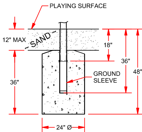
SAND-FILLED FOOTING * DEPENDING ON SAND DEPTH (SHOWN ABOVE)
