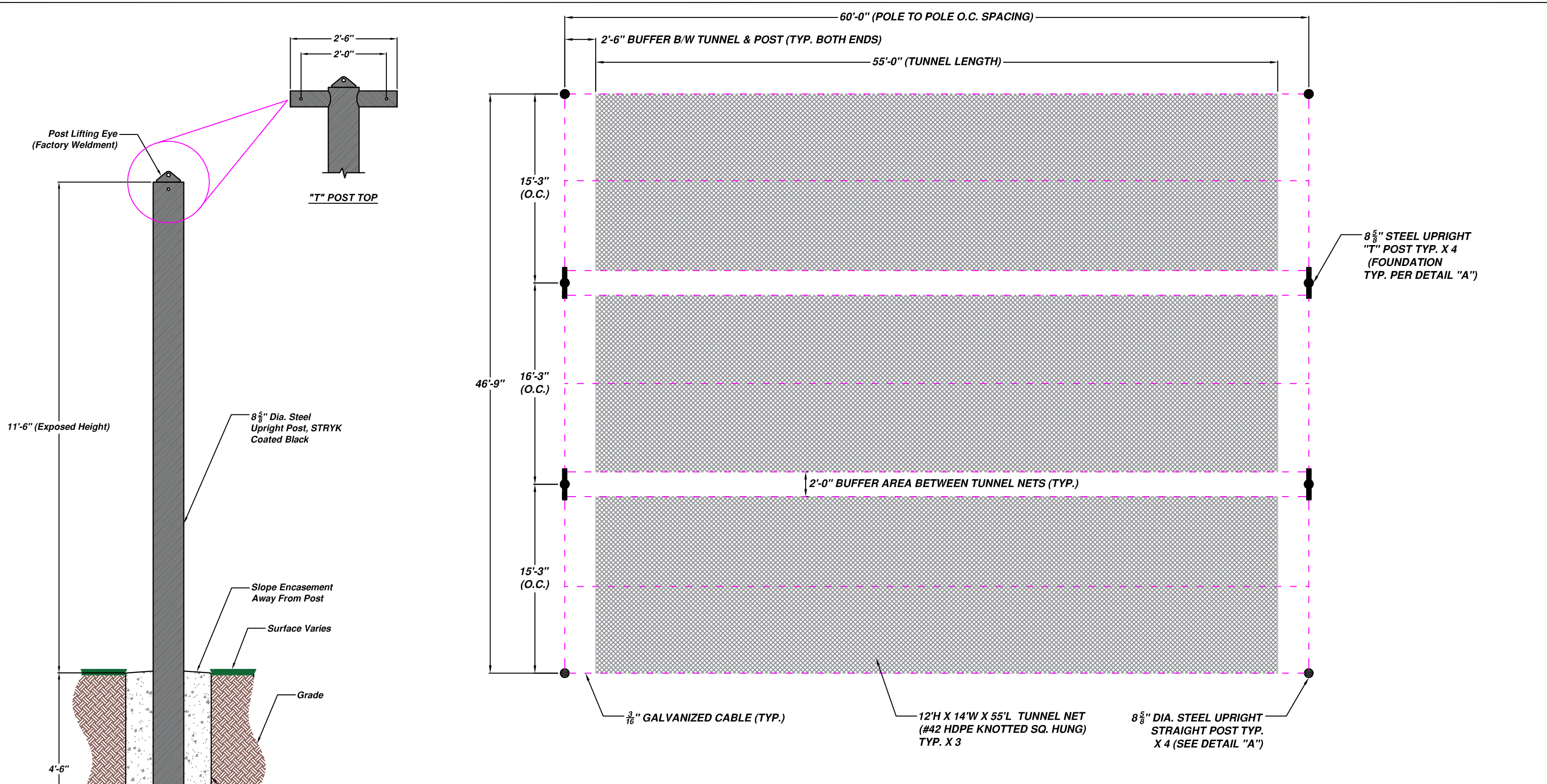
TRIPLE POWERHOUSE SOFTBALL BATTING CAGE - PLAN VIEW (SPORTSEGE® PART # SETSBC-01)
