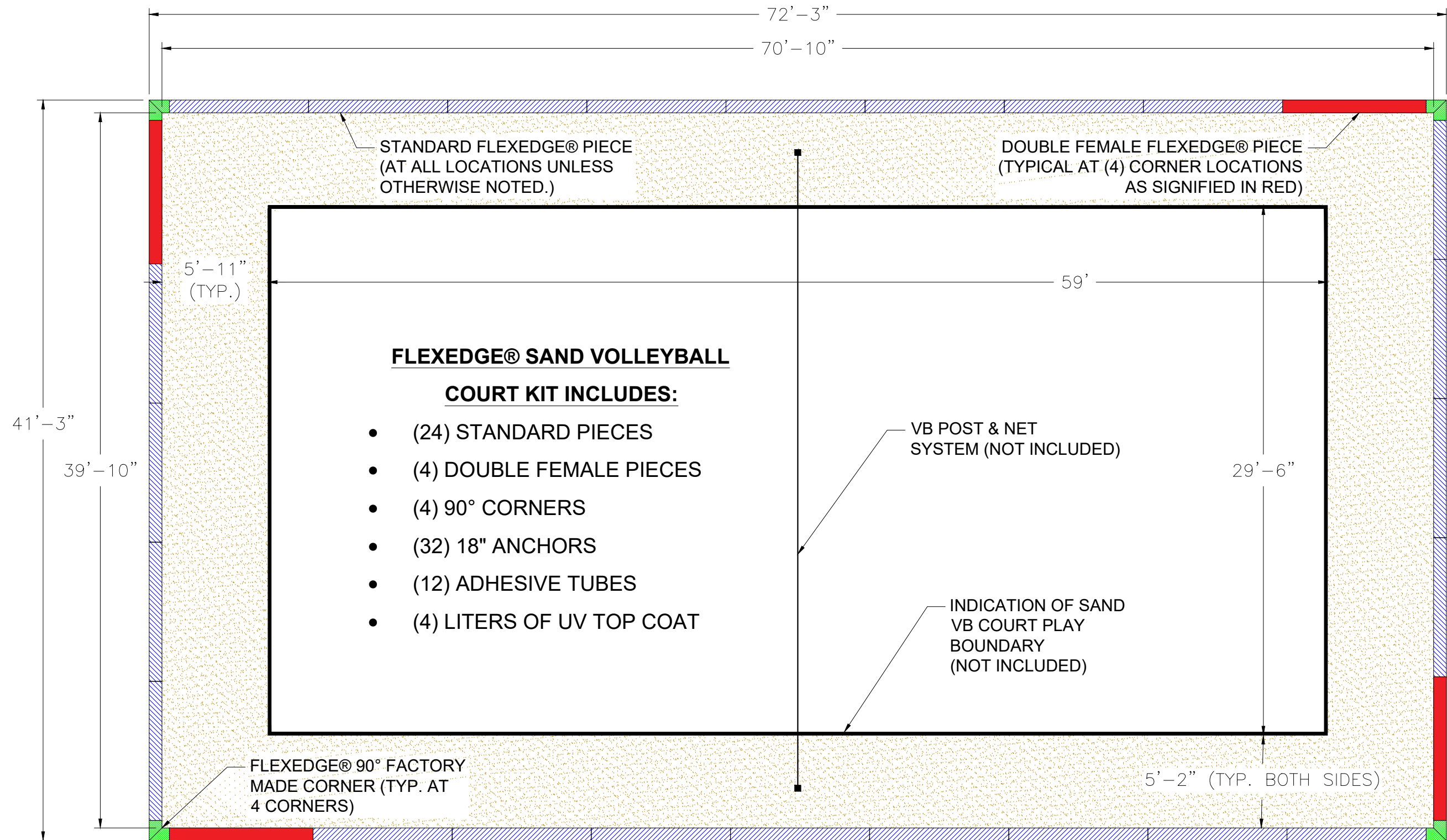
FLEXEDGE® SMALL VOLLEYBALL CURB KIT LAYOUT
