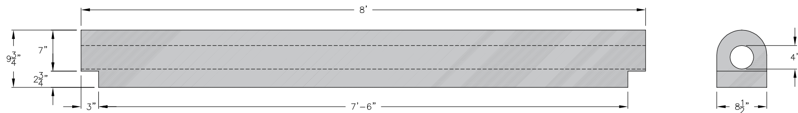
CUSTOM FLEXEDGE® VOLLEYBALL CURB
