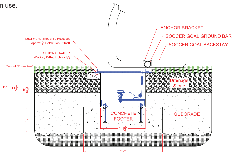
SEF790 - SOCCER GOAL ANCHOR FRAME INSTALLATION DETAIL
