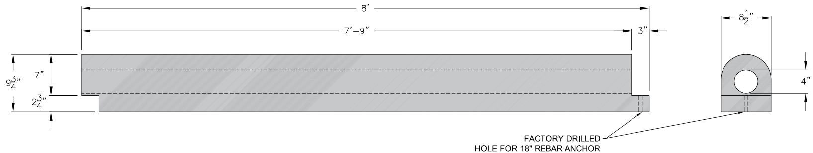
STANDARD FLEXEDGE® VOLLEYBALL CURB
