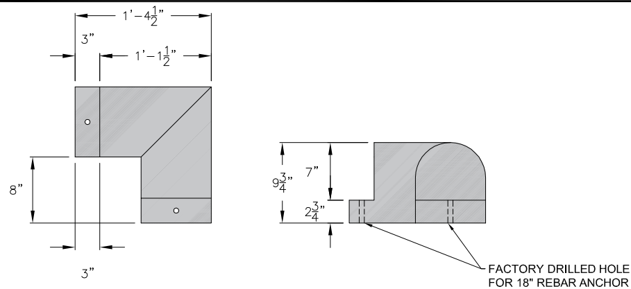
FLEXEDGE® VOLLEYBALL CURB CORNER
