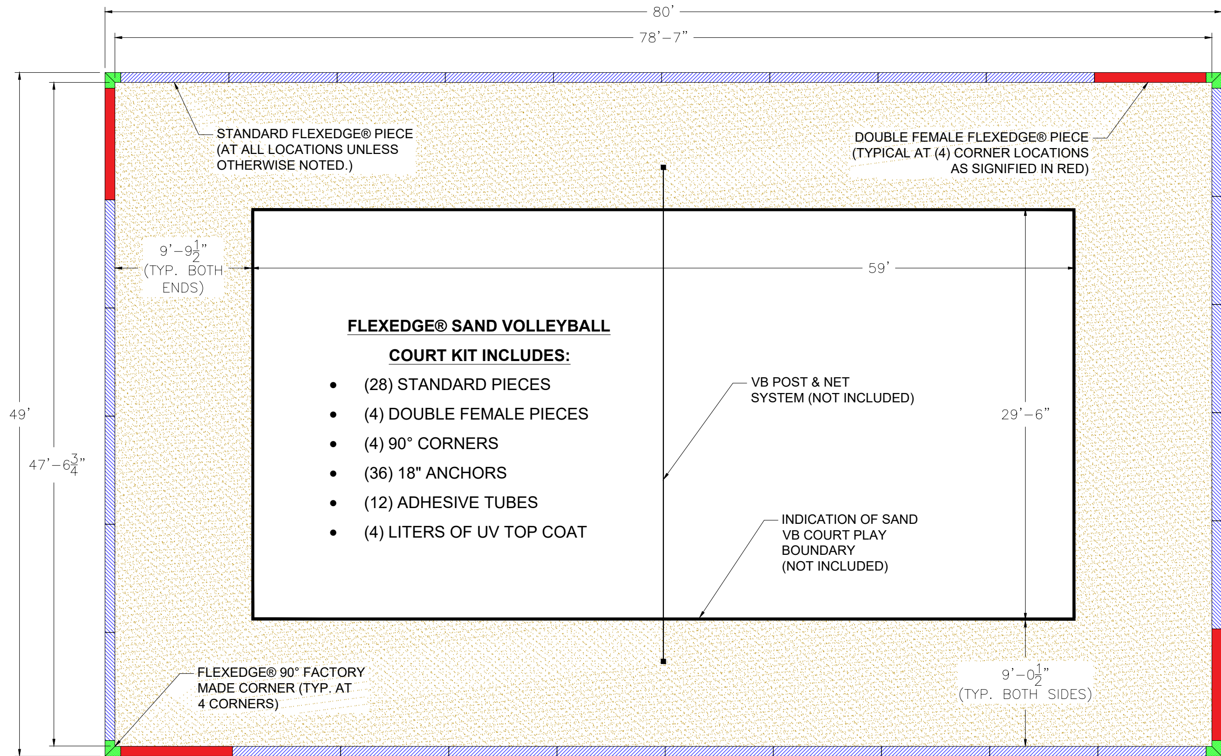
FLEXEDGE® STANDARD VOLLEYBALL CURB KIT LAYOUT
