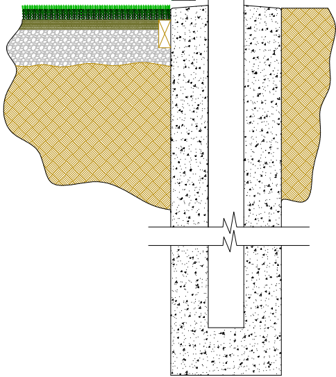
DiamondWall Typical Installed Cross Section
