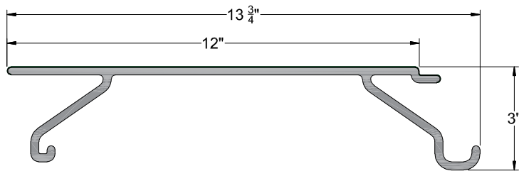
DiamondWall Individual Extruded Panel - Cross Section (Part # SE.DWP)
