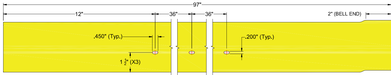
DiamondWall StadiumGuard Top Cap - Front View (Part # SE.DWH)
