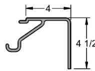
Right (Male) End Cap (Part # SE.DWP.ECM)
