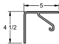
Left (Female) End Cap (Part # SE.DWP.EFM)
