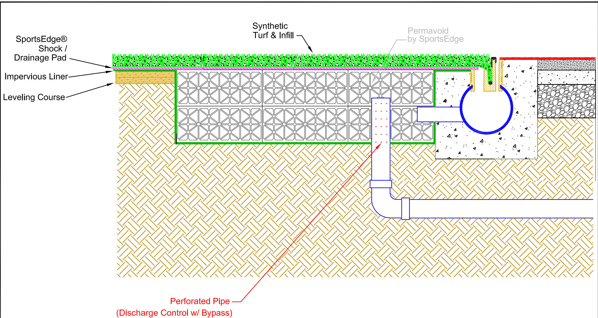
Plan View- SportsEdge Terminator Drain System w/ Permavoid Water Control System
